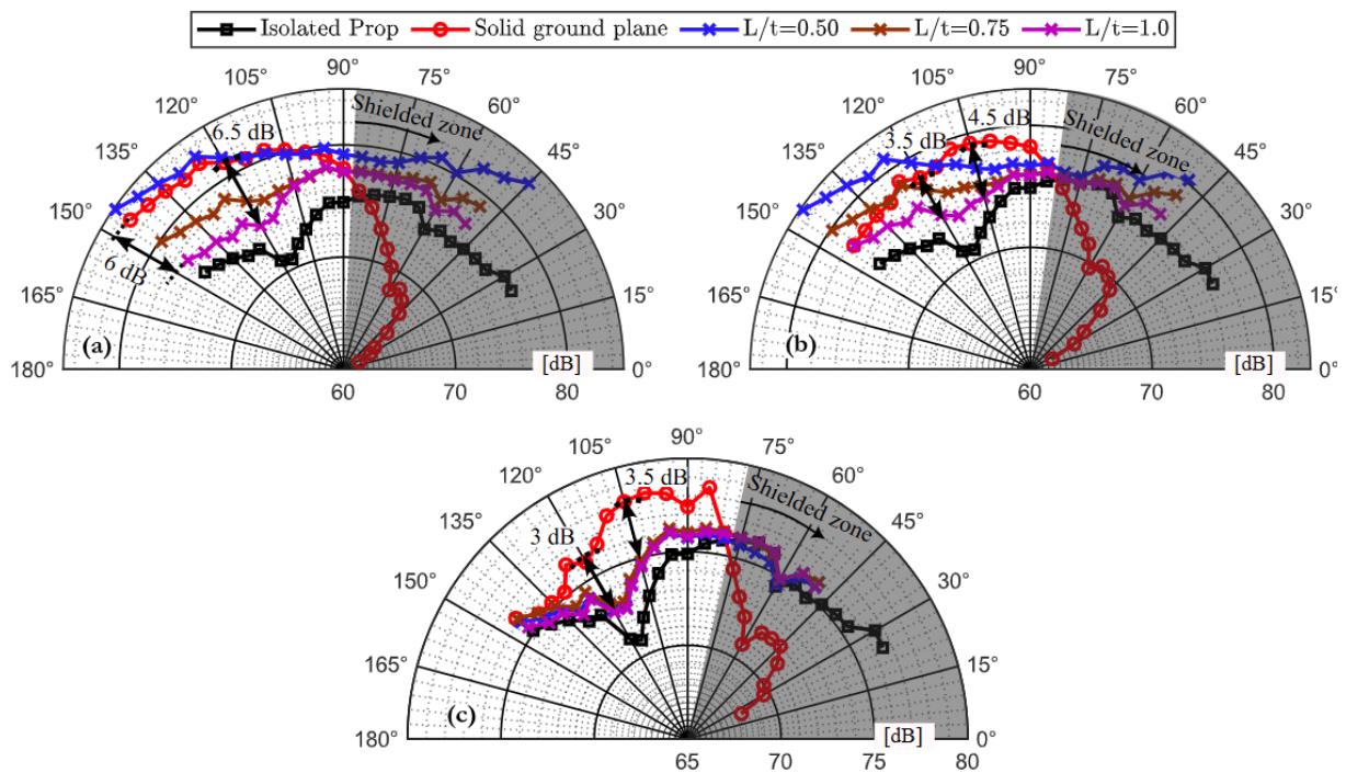
Fig. 1: The far-field OASPL directivity for propeller in various L/t
