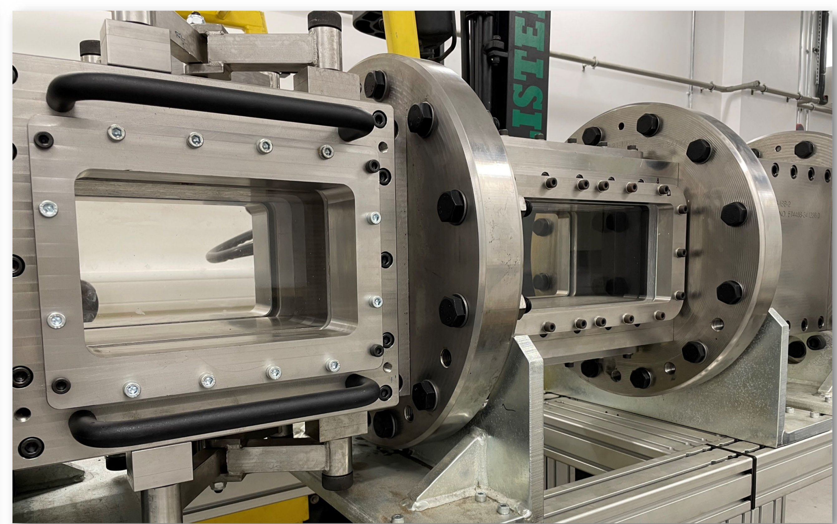
Modular test section with optical access
